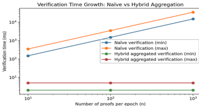
Fig3. Verification time versus number of proofs per cycle n . Simple verification increases linearly with n , while hybrid iterative pooling results in a quasi-constant (or logarithmic) verification cost.
